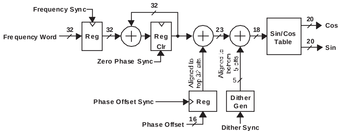
Figure 31. Transmit NCO
