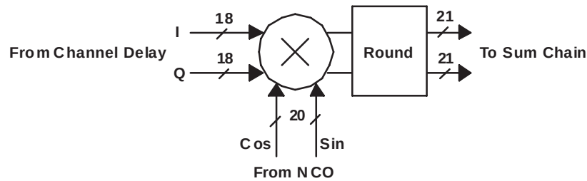
Figure 30. Transmit Mixer
